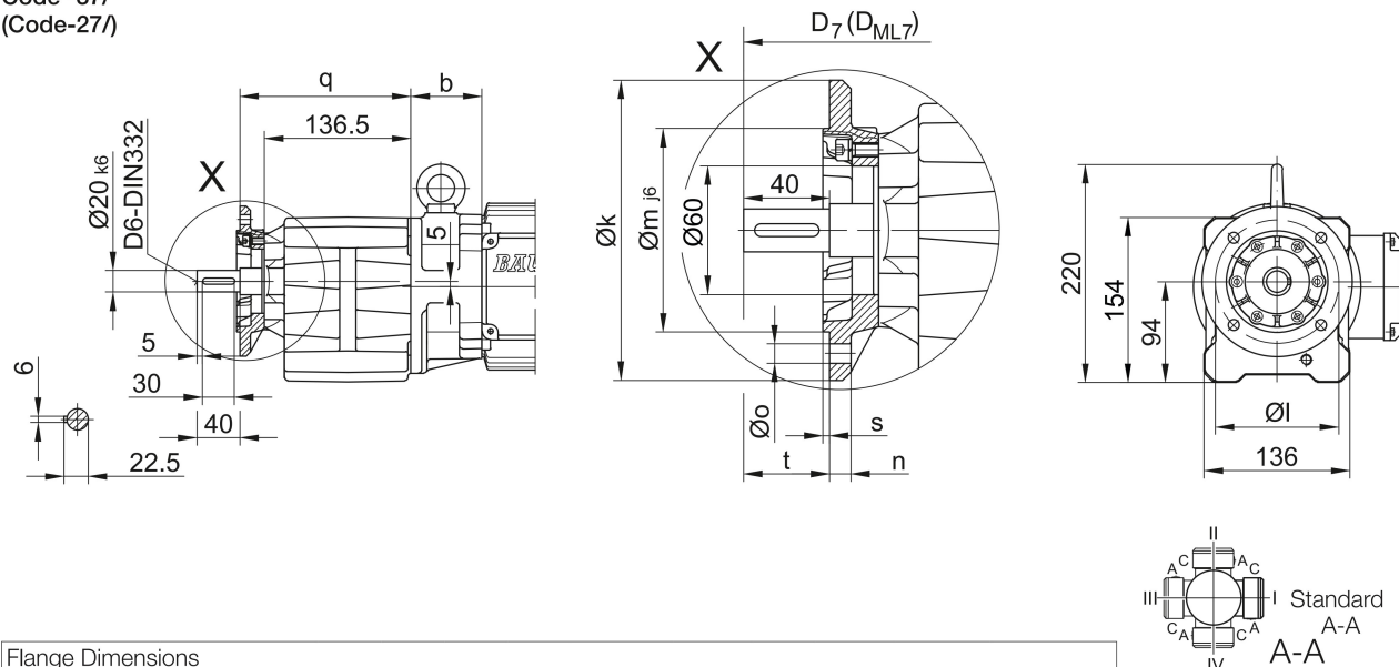
Flange Dimensions
